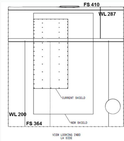
Ice Shield Technical Drawings
