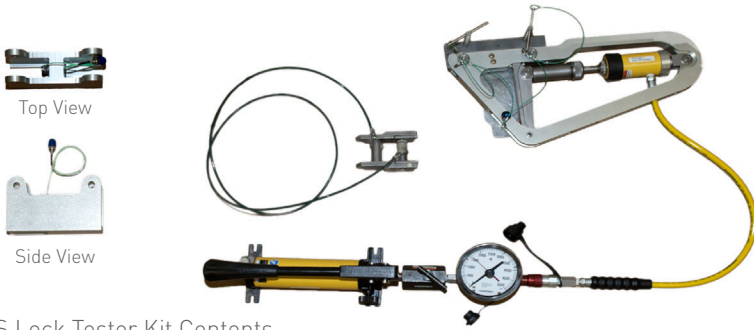
ECHS Lock Tester Kit Contents
