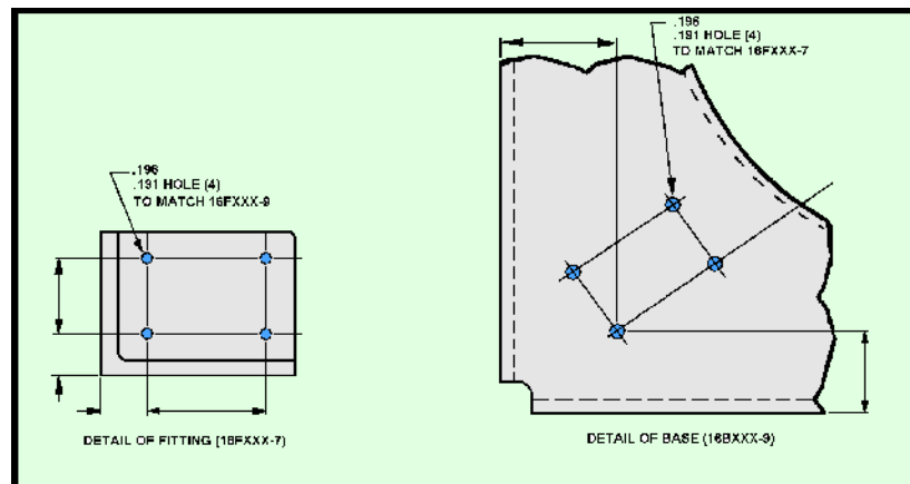
Figure 13. Example of “To Match” hole patterns as defined on engineering drawings. 7.0 SHIPPING AND STORAGE CONTAINERS FOR BUYER FURNISHED TOOLS
