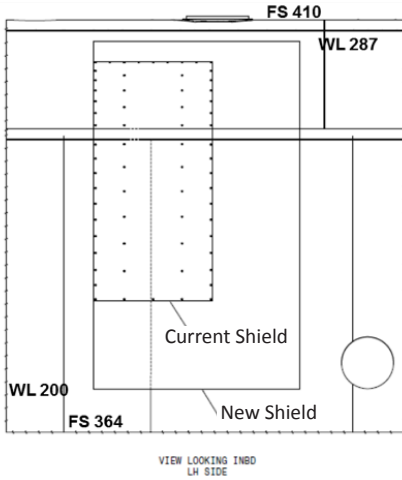
Ice Shield Technical Drawings
