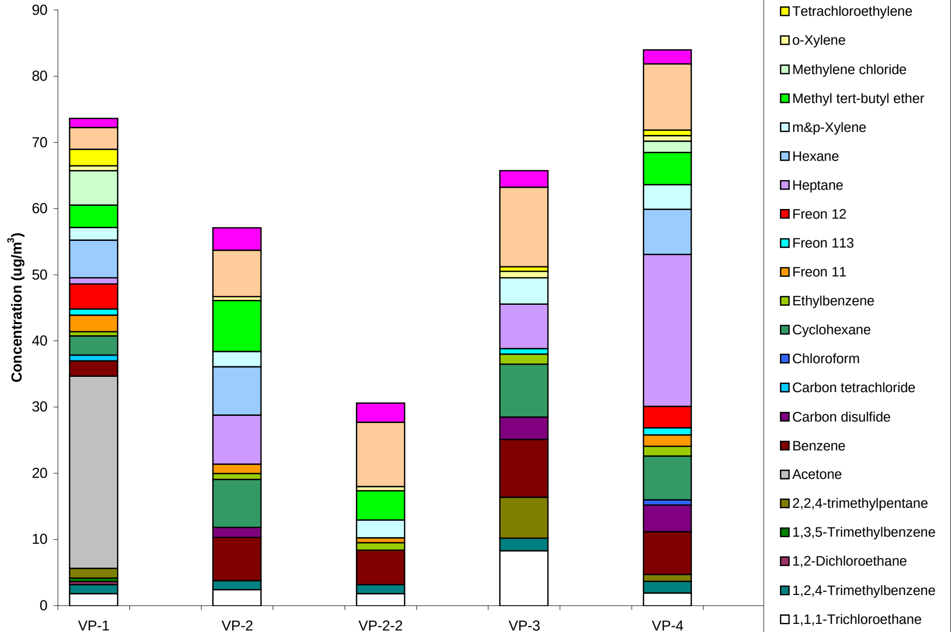
Figure 3. Soil Gas Concentrations of Constituents Detected at the West Lot Site.
