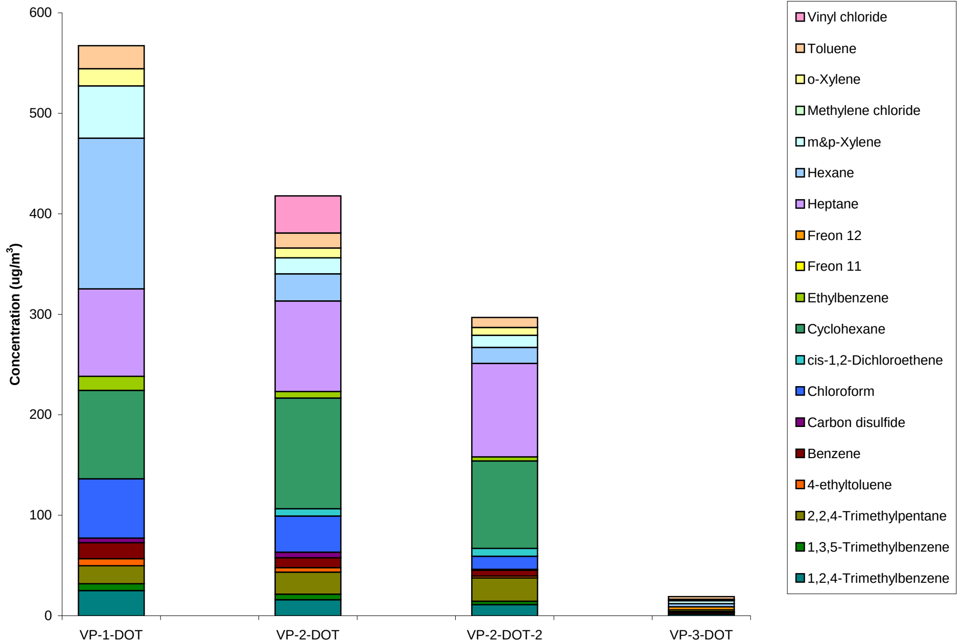
Figure 4. Soil Gas Concentrations of Constituents Detected at the DOT Property.
