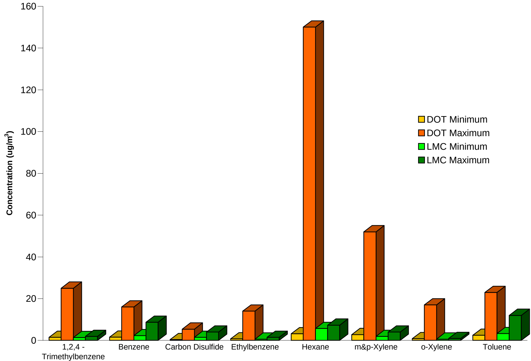
Figure 5. Comparison of Compounds Detected in All Samples From the DOT Property to Compounds Detected in Samples From the West Lot Site.
